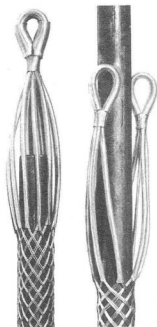
Model DLE Dual lift with suspension lift eyes.
